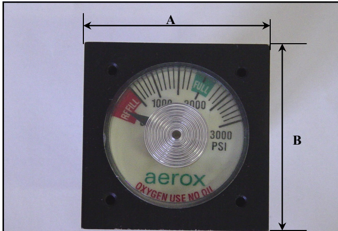
4110-489, Panel Mount Gauge (Front)
