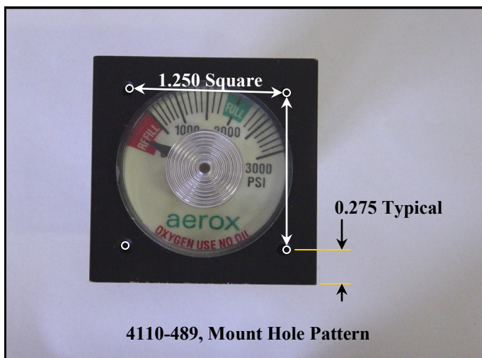
4110-489, Panel Mount Gauge (Side)
